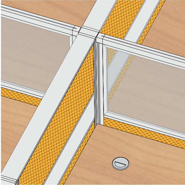
Hybrid Model : Piazza – MXI hybrid Main Spine : Piazza 65mm Divider : MXI 25mm
