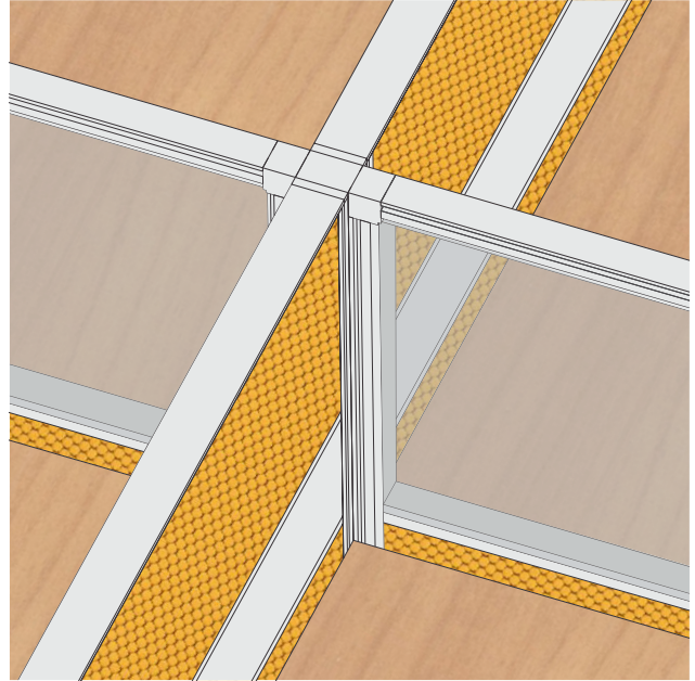
Hybrid Model : Molex – Hazi hybrid Main Spine : Molex 50mm Divider : Hazi 30mm
